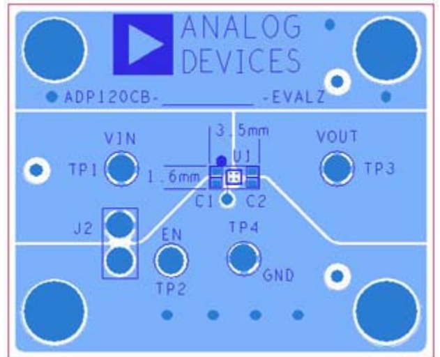
Figure 49. WLCSP PCB Layout—Top Side
