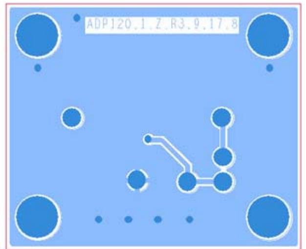
Figure 50. WLCSP PCB Layout—Bottom Side
